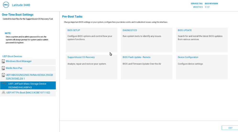
Figure 10. Boot Menu
