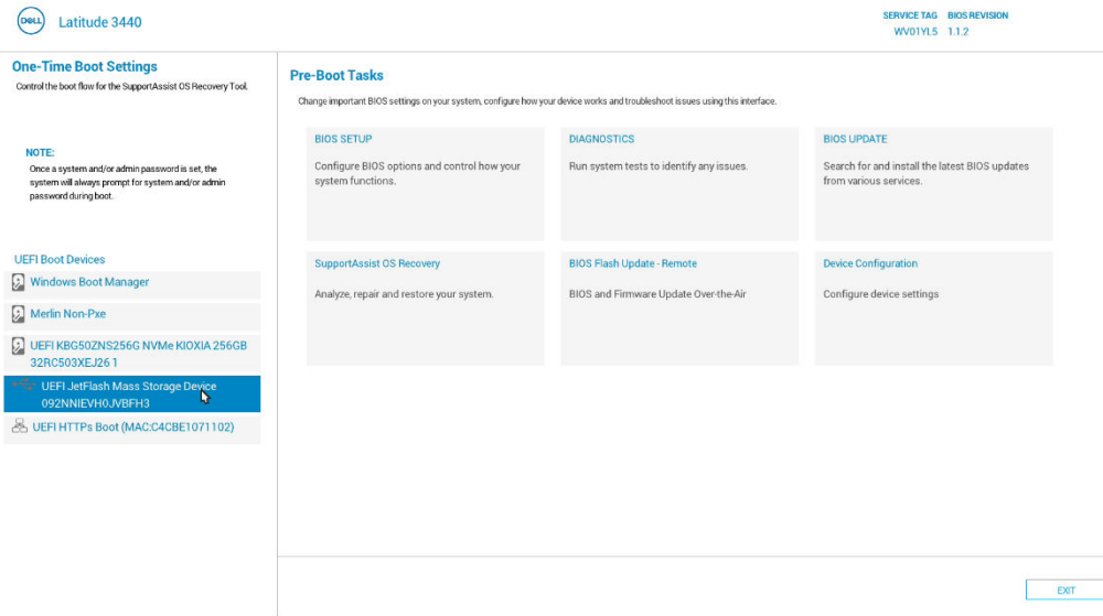
Figure 12. Pre-Boot tasks
