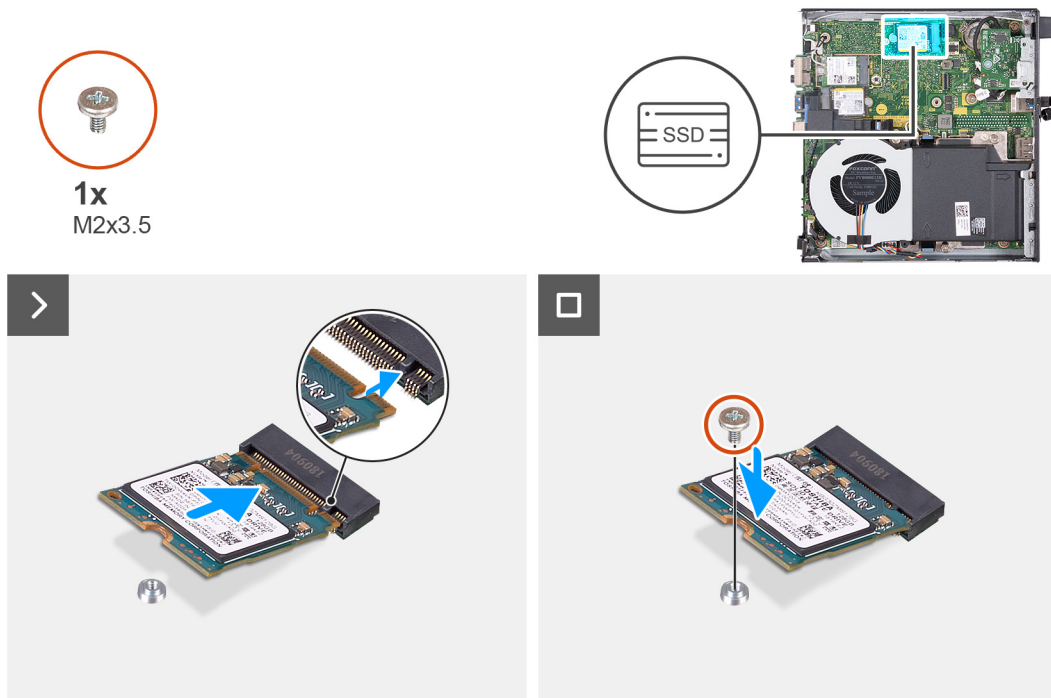
Figure 22. Installing the M.2 2230 solid-state drive in slot 1
