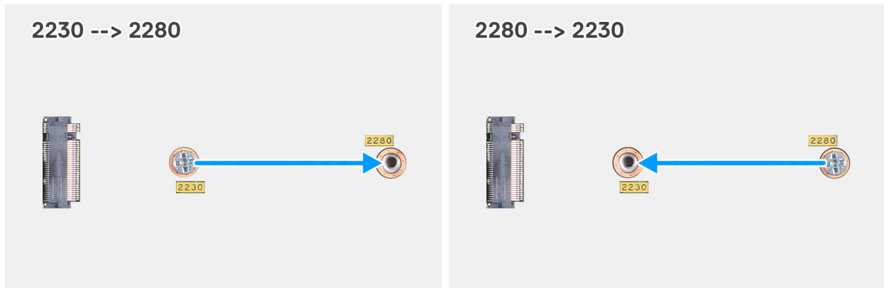
Figure 27. Moving the screw mount to support a different form factor (OptiPlex Micro Plus 7020)
