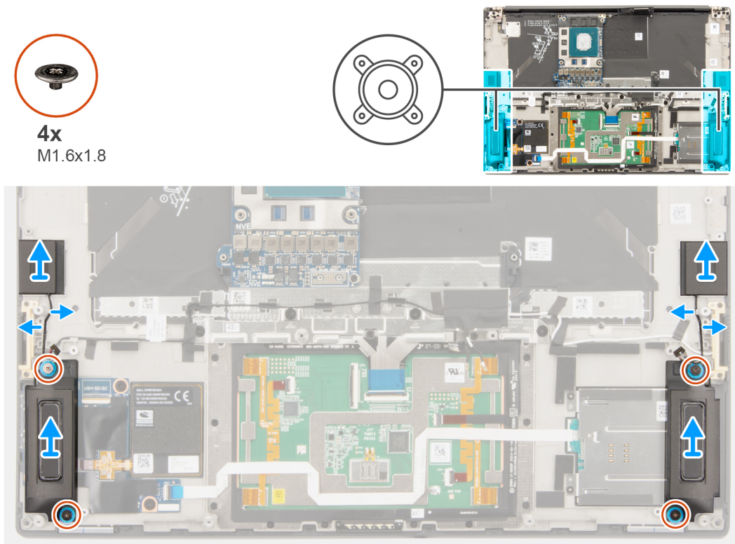
Figure 68. Removing the speakers
