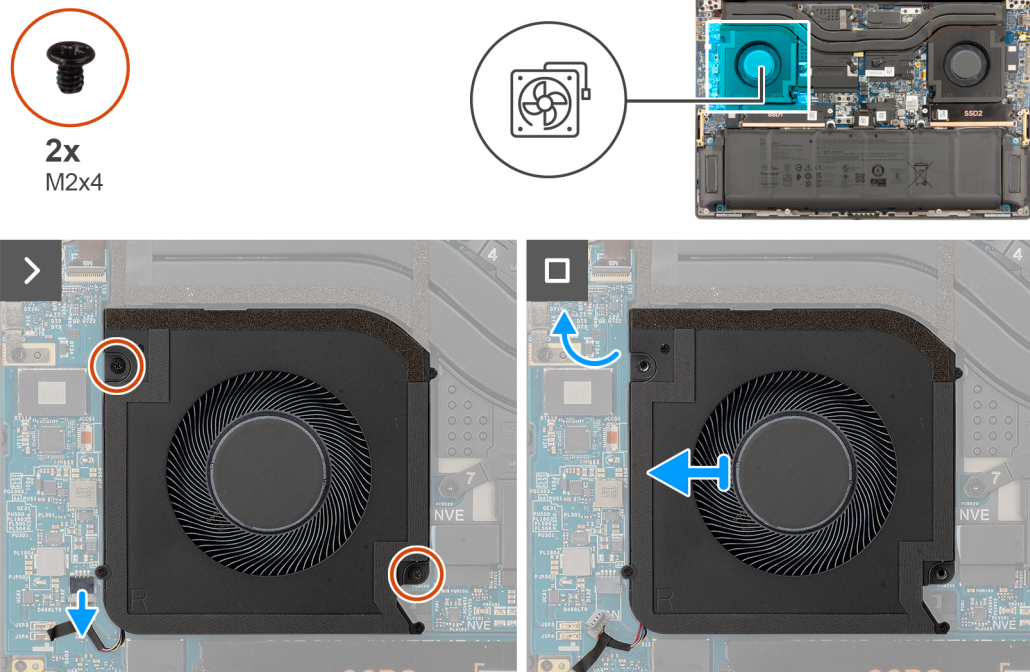
Figure 24. Removing the graphics-card fan
