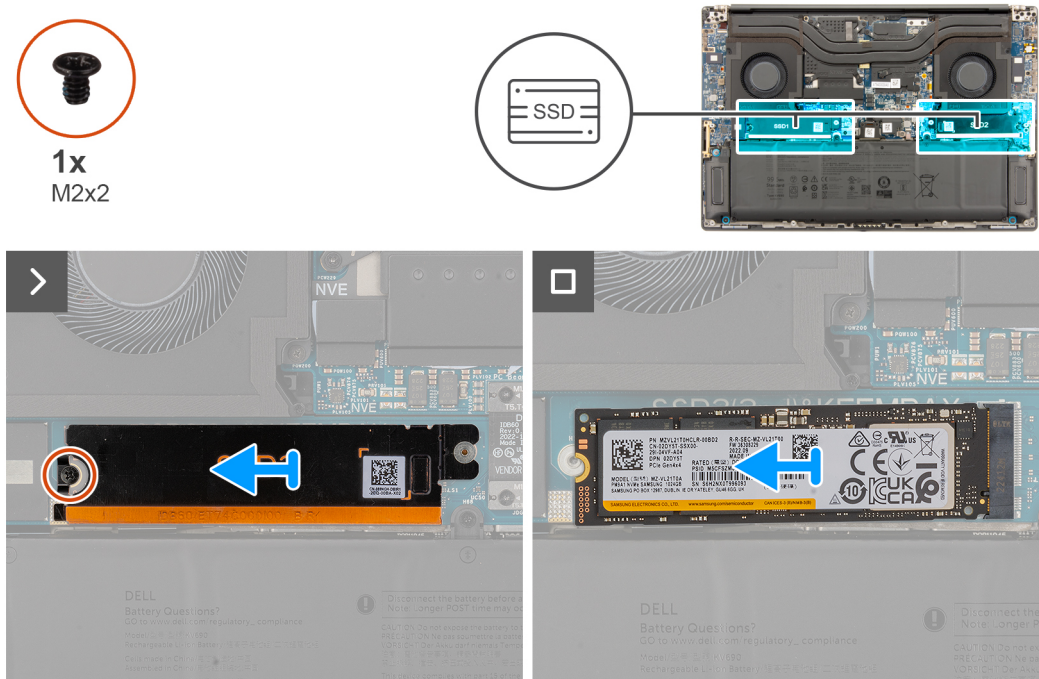
Figure 18. Removing the M.2 2280 SSD
