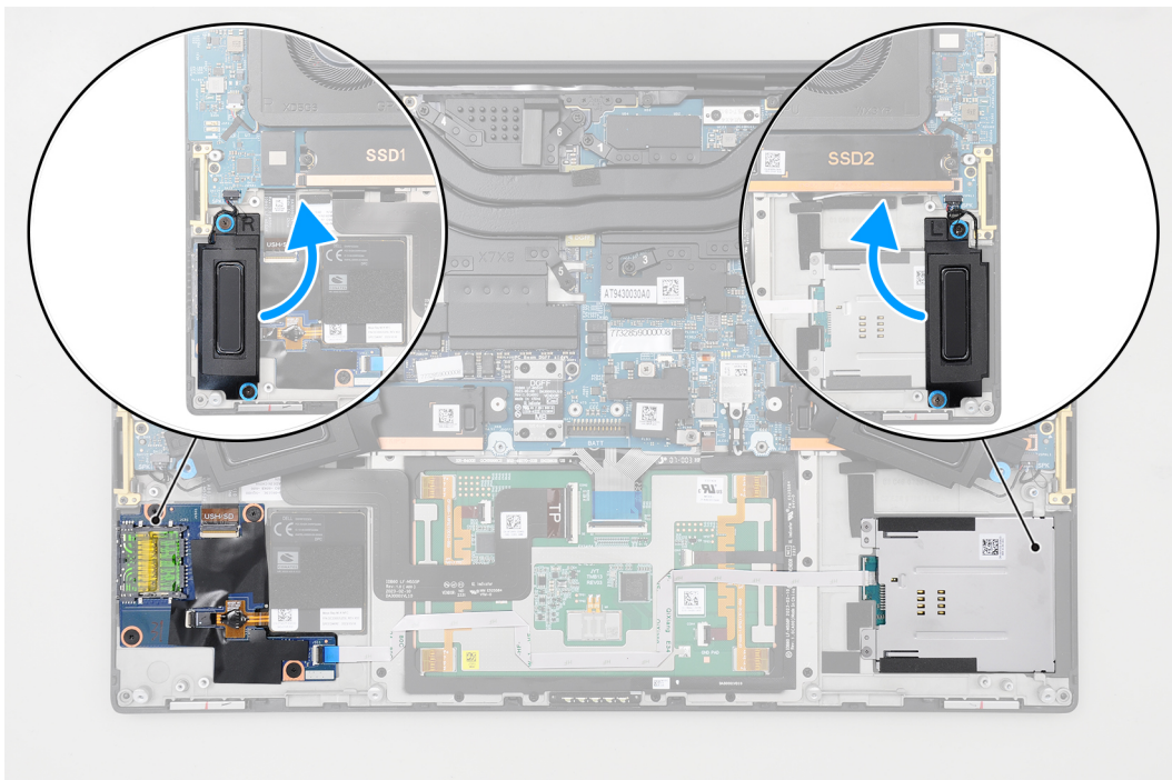
Figure 38. Speakers
