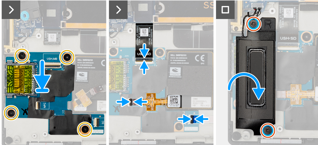
Figure 42. Installing the USH and SD-card daughterboard
