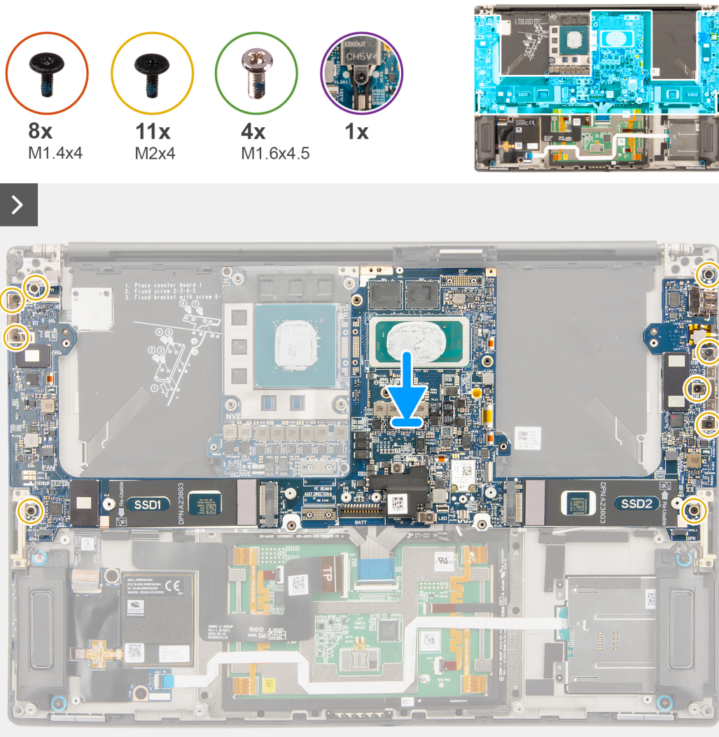
Figure 63. Installing the system board
