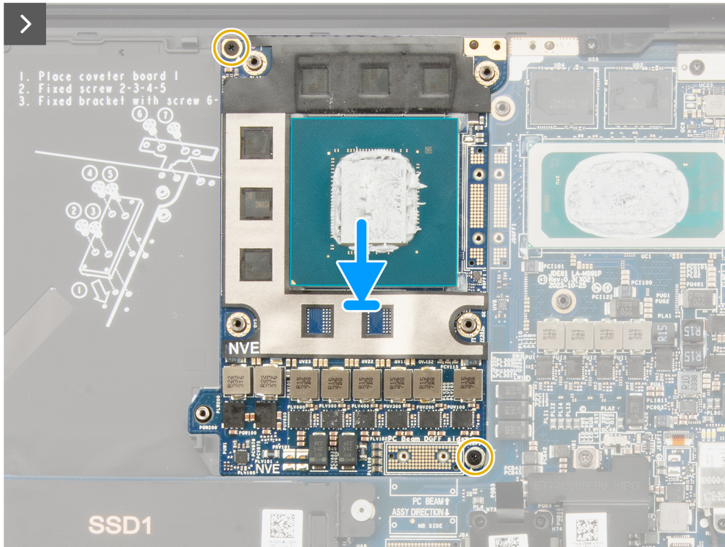
Figure 47. Removing the graphics card
