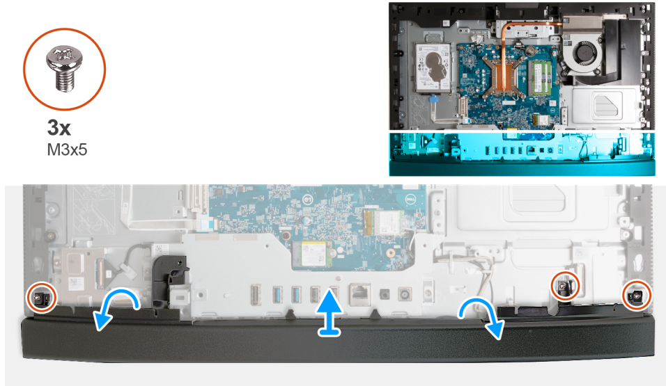
Figure 99. Removing the bottom cover
