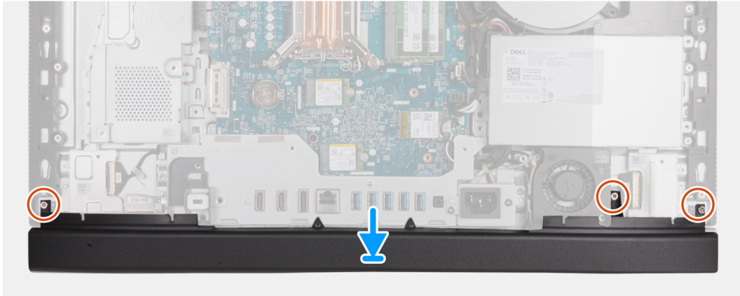
Figure 45. Installing the bottom cover
