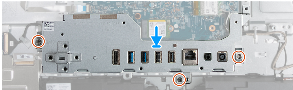
Figure 106. Installing the I/O bracket
