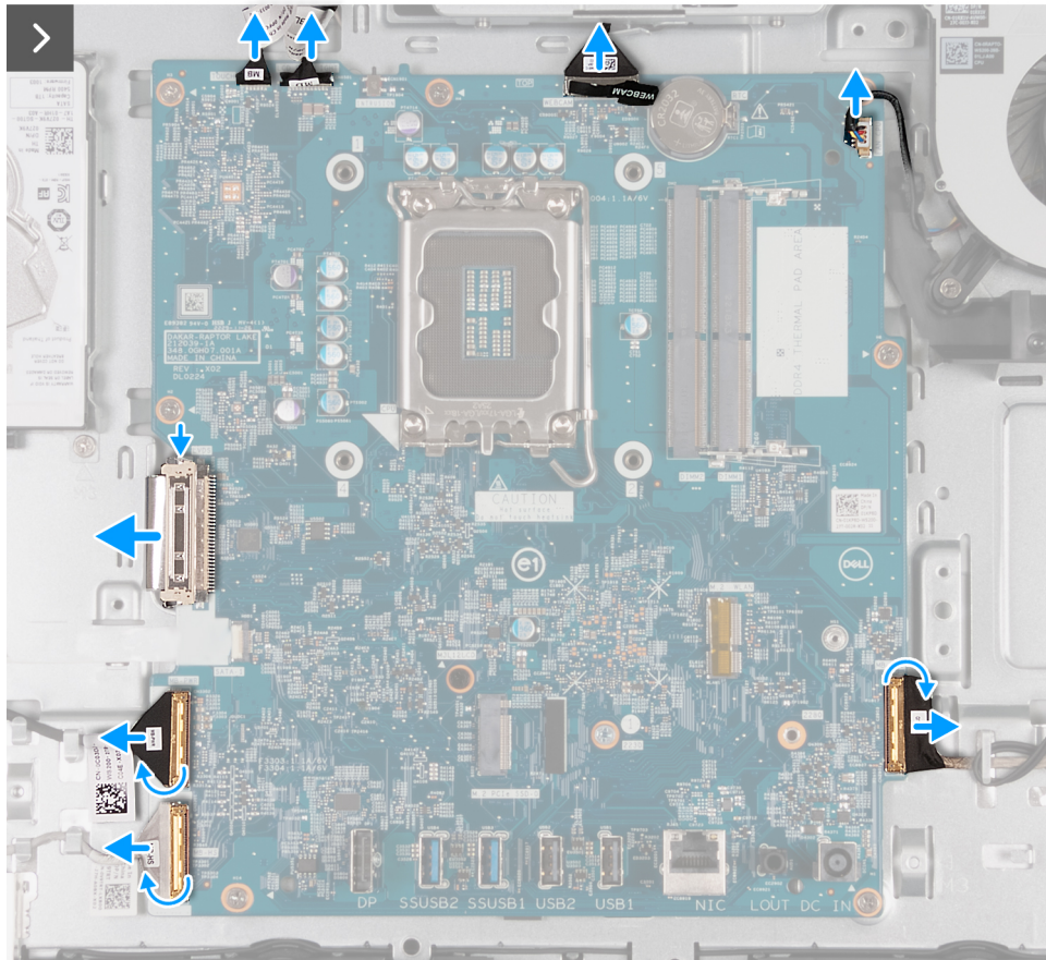
Figure 114. Removing the system board
