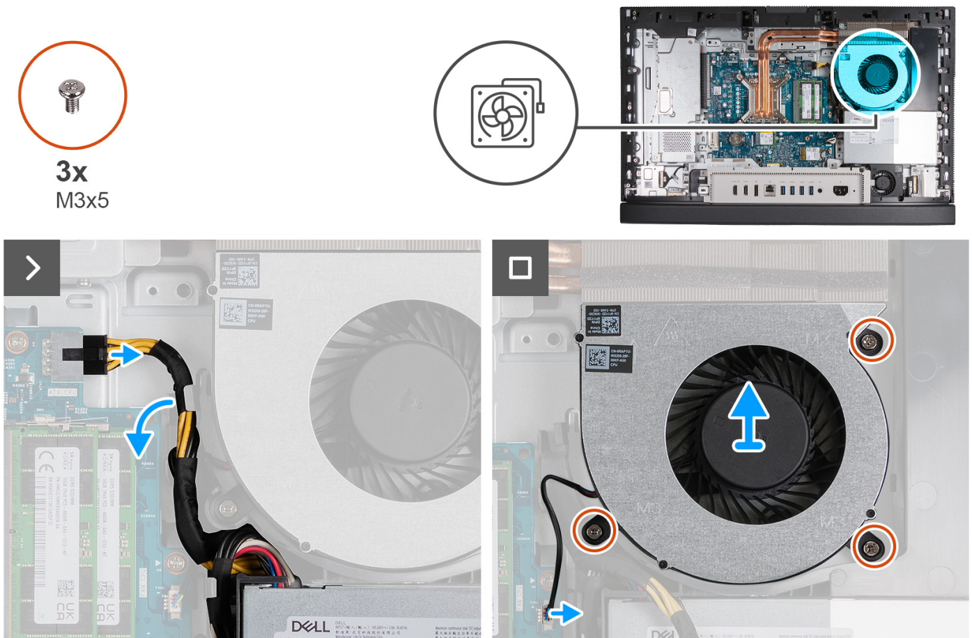
Figure 48. Removing the fan
