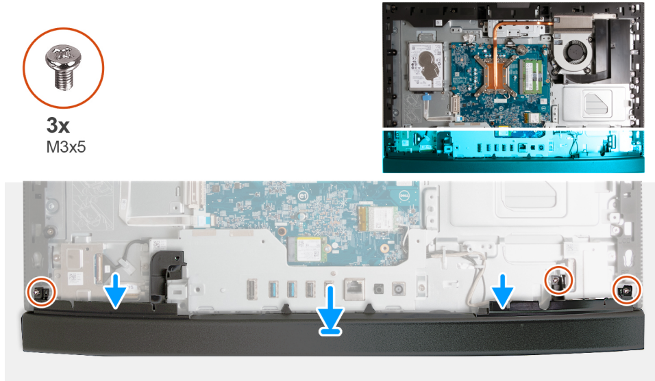
Figure 100. Installing the bottom cover
