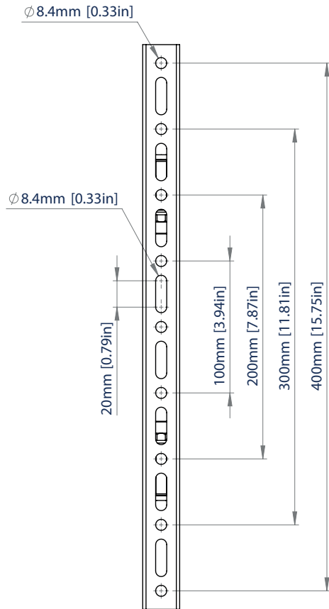
FRONT VIEW
