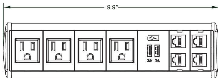
Model: SYM-CL-4AC-1CA-2SS
