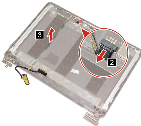
Figure 35. Disconnect and remove the EDP cable
