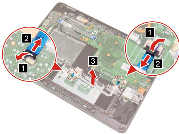
Figure 22. Disconnect and remove the touchpad cable
