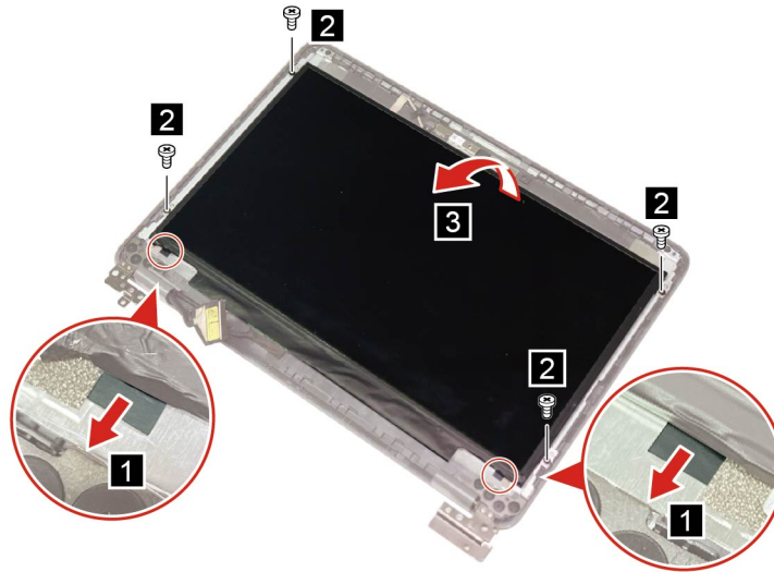
Figure 31. Pull out two pieces of the removable tape and remove four screws
