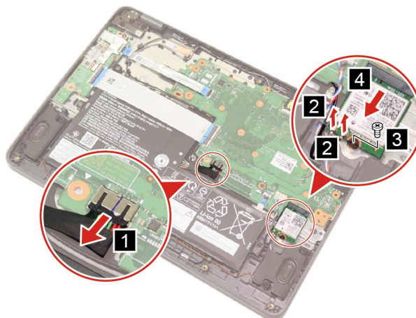
Figure 16. Disconnect the battery pack cable and remove the Wi-Fi card
