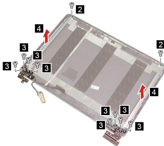
Figure 37. Remove ten screws and the hinges
