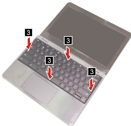
Figure 10. Install the keyboard
