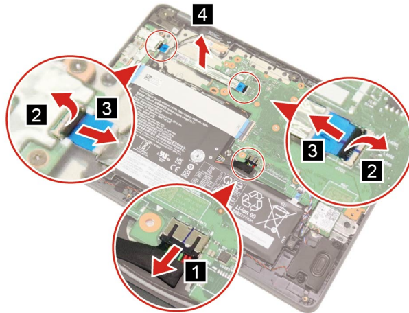
Figure 13. Remove the 14-pin I/O board cable
