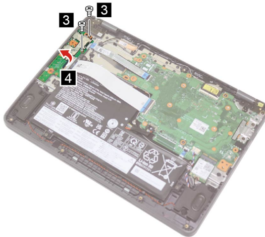
Figure 20. Remove two screws and the I/O board
