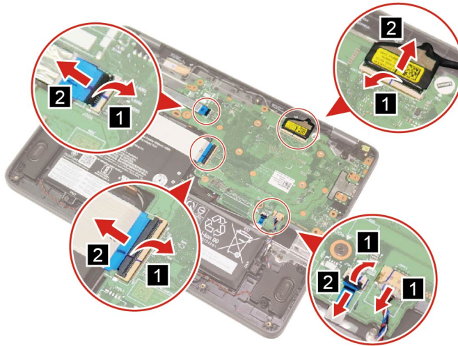
Figure 23. Disconnect all cables
