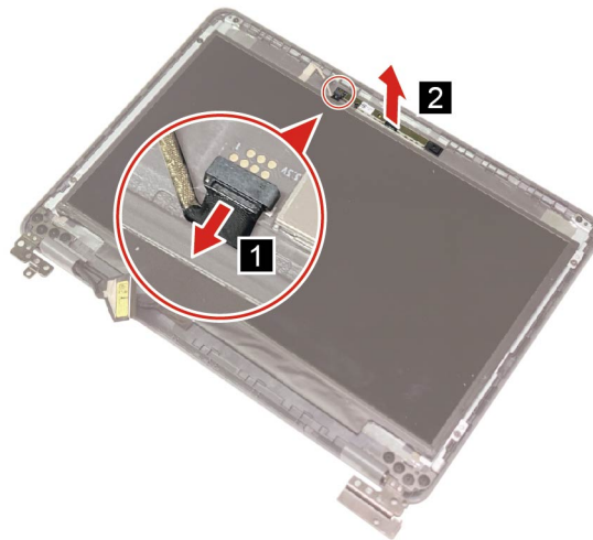
Figure 33. Disconnect the camera cable and remove the camera board
