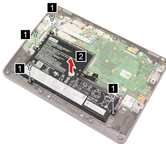
Figure 15. Remove four screws and the battery pack
