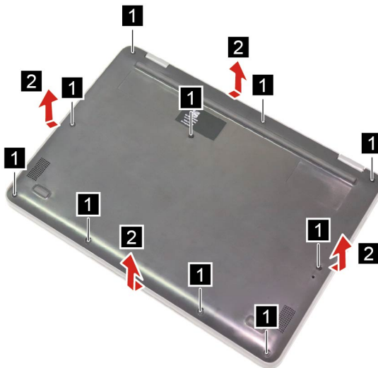
Figure 12. Loosen ten screws and remove the lower case
