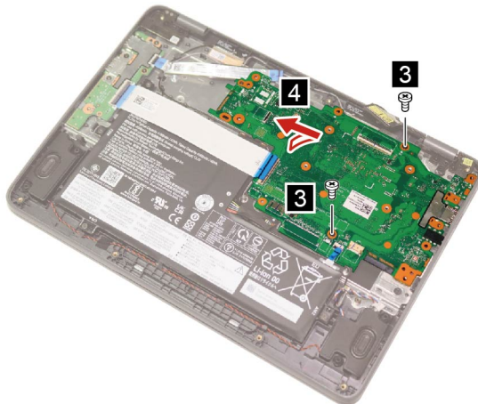
Figure 24. Remove two screws and the system board
