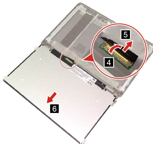
Figure 32. Disconnect the EDP cable and remove the LCD panel
