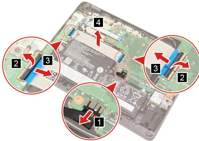
Figure 14. Remove the 40-pin I/O board cable
