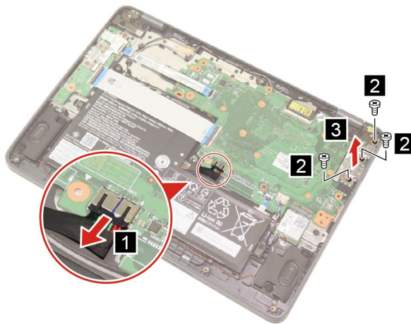
Figure 21. Remove the Type-C bracket
