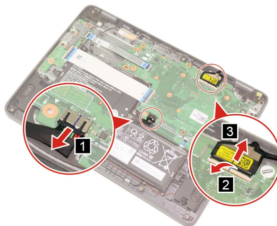
Figure 27. Disconnect the battery pack cable and LCD cable from the system board
