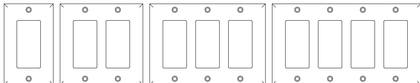
SS-DPLT1 1 Gang Style Wall Plate SS-DPLT2 2 Gang Style Wall Plate SS-DPLT3 3 Gang Style Wall Plate SS-DPLT4 4 Gang Style Wall Plate
