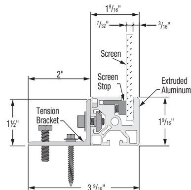
VERSAROLL dimensions
