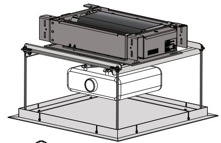
AeroLift 35 shown with optional small closure panel
