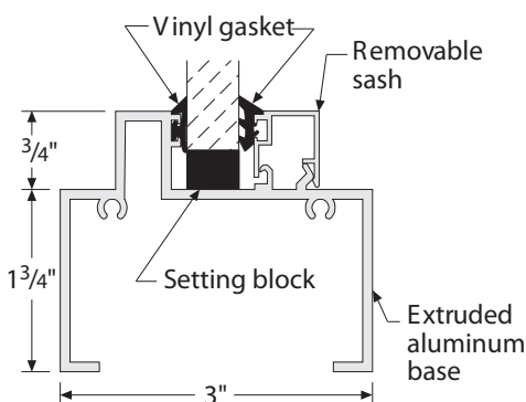
SYSTEM 200 dimensions
