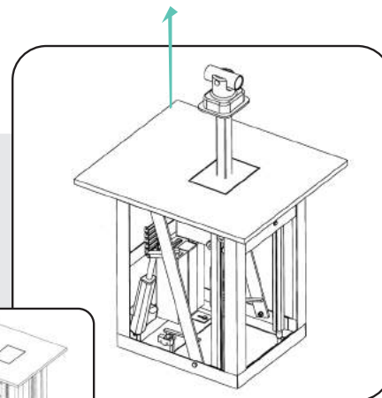
Videoconferencing camera concealed in table, then raised for use.
