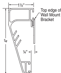
Frame Extrusion Side Detail
