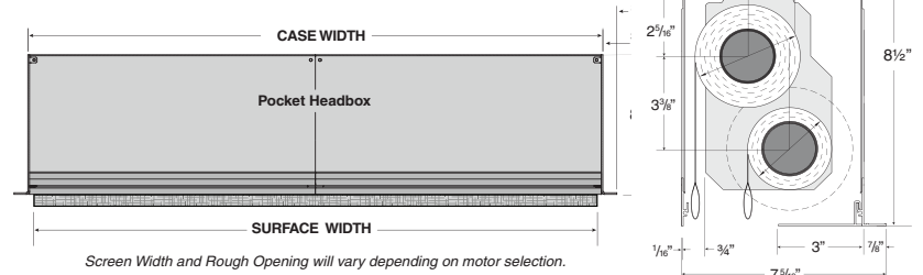
Large Dual Roller Screen with Pocket Headbox - Dimensions Motorized Only
