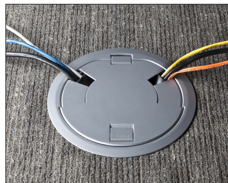
Cables egress from a CRFB Series Floor Box with Evolution Series Poke-Thru Cover.
