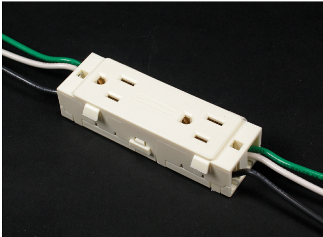
15A replacement device. 6" (152mm) wire leads each side.
