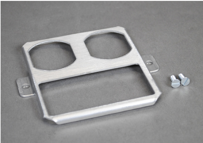
Duplex and GFI openings faceplate.
