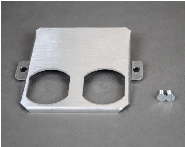
Single duplex opening faceplate.
