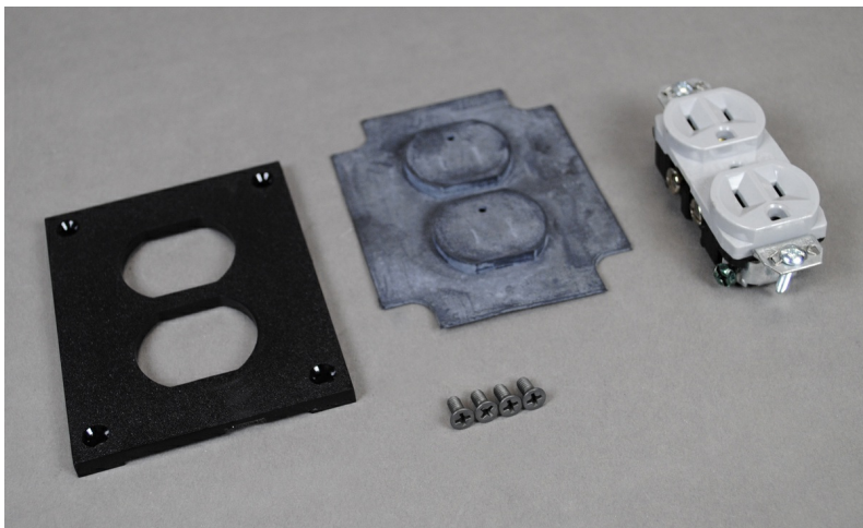
Nonmetallic double duplex membrane cover plate.
