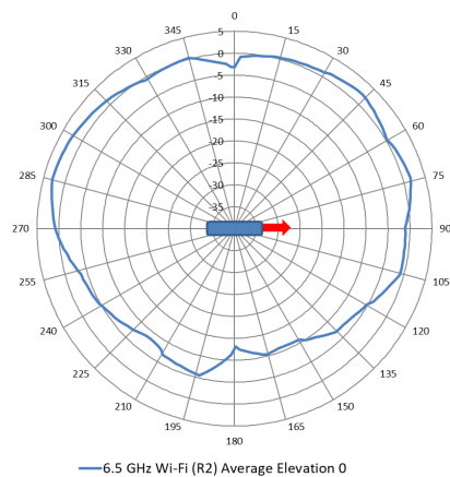
Figure 8. 6.5 GHz Wi-Fi antenna patterns (vertical) with elevation 0
