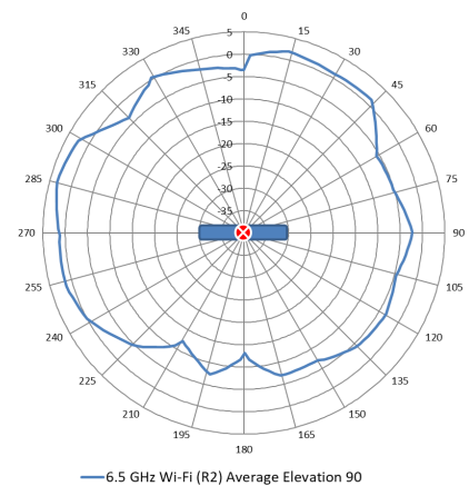
Figure 9. 6.5 GHz Wi-Fi antenna patterns (vertical) with elevation 90
