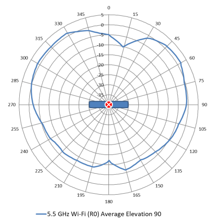
Figure 7. 5.5 GHz Wi-Fi antenna patterns (vertical) with elevation 90
