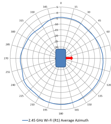
Figure 1. 2.45 GHz Wi-Fi antenna patterns (horizontal) for both 2.4 GHz + 5 GHz mode and 2.4 GHz + 6 GHz mode
