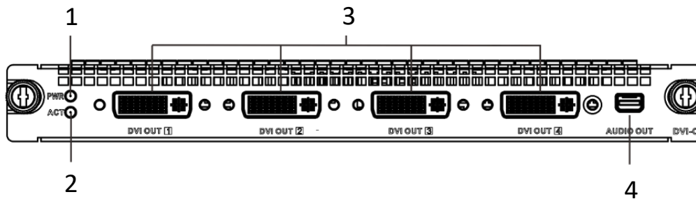
Figure 1-9 Front View of DVI Output Board
