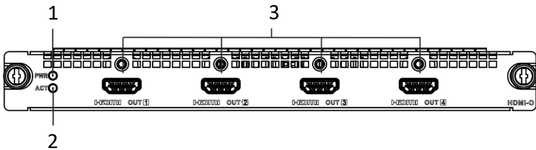
Figure 1-11 Front View of HDMI Output Board
