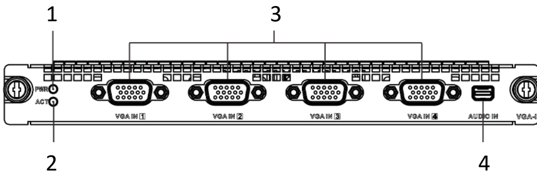
Figure 1-5 Front View of VGA Input Board
