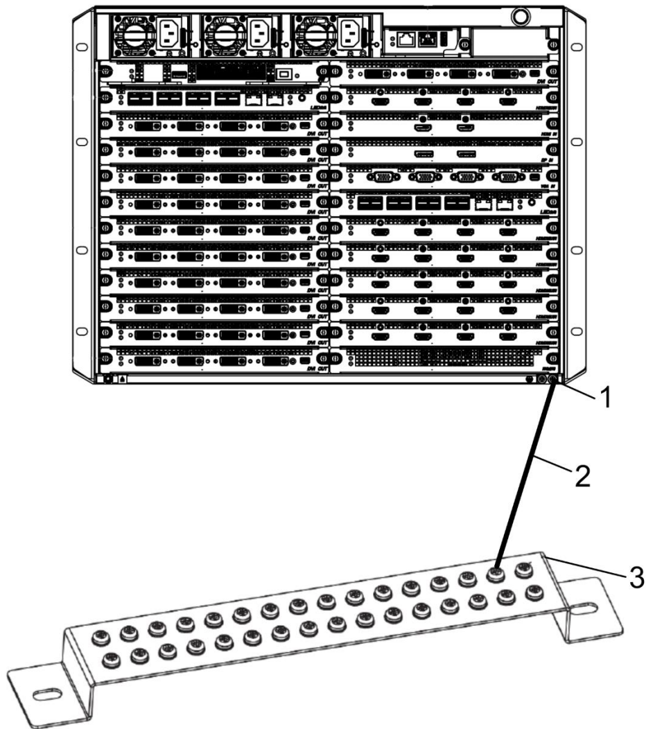
Figure 2-5 Connect the Grounding Cable to the Grounding Row
