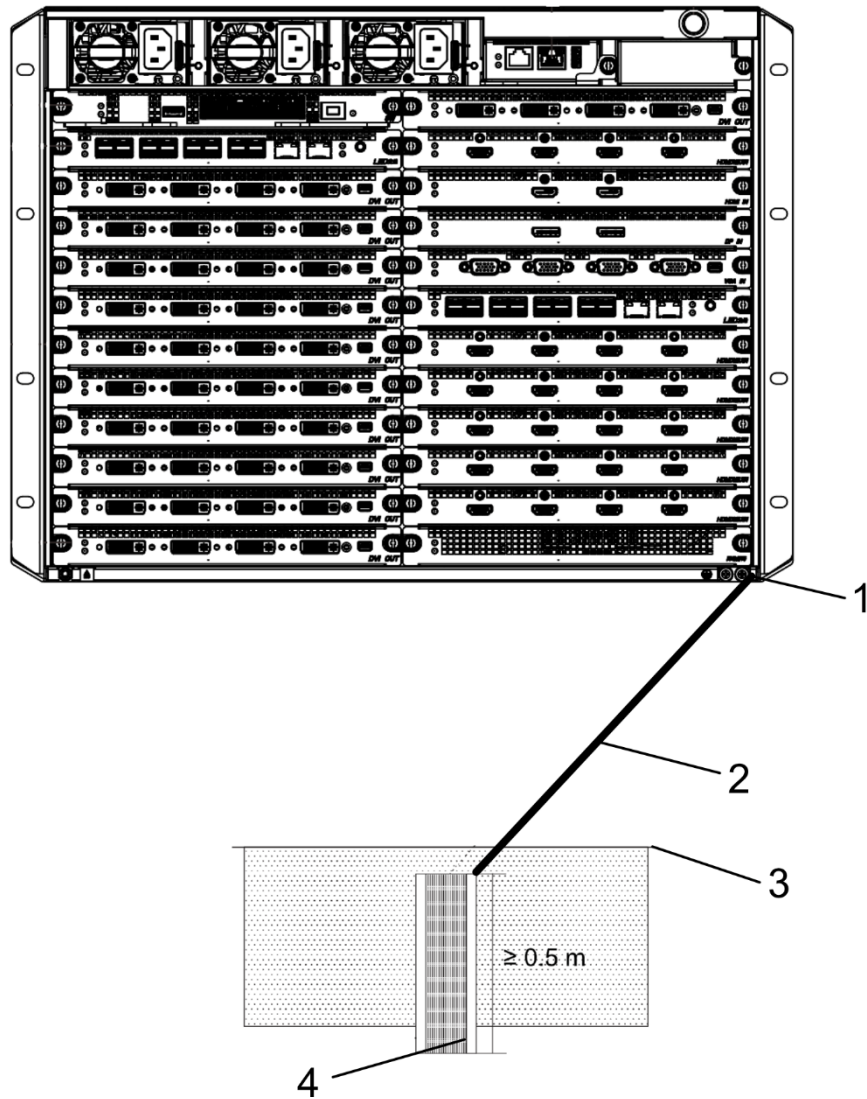
Figure 2-6 Connect the Grounding Cable to the Ground
