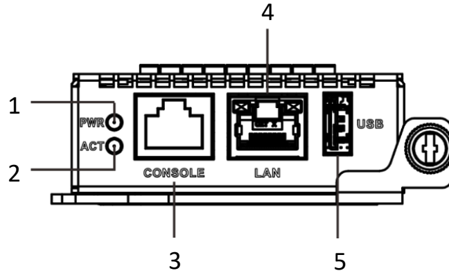
Figure 1-3 Front View of Main Control Board
