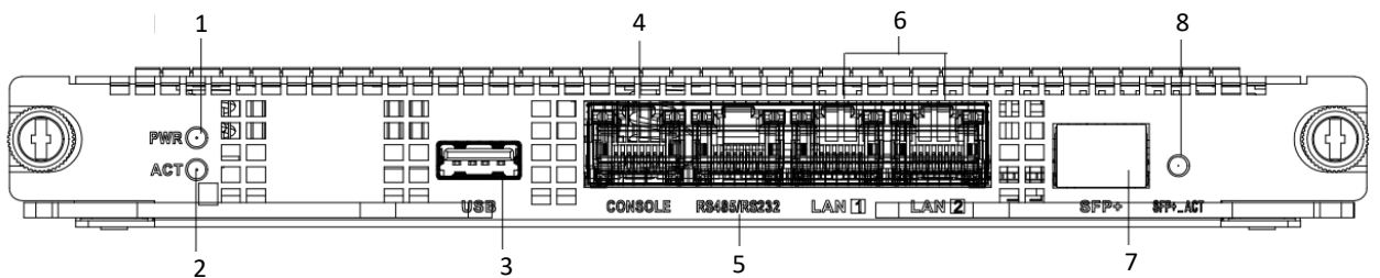
Figure 1-4 Front View of Switch Board
