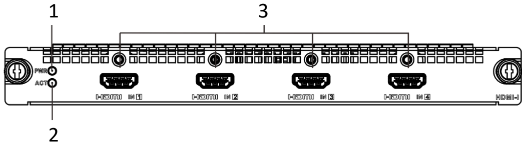
Figure 1-10 Front View of HDMI Input Board
