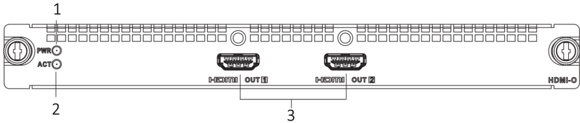
Figure 1-12 Front View of HDMI UHD Output Board
