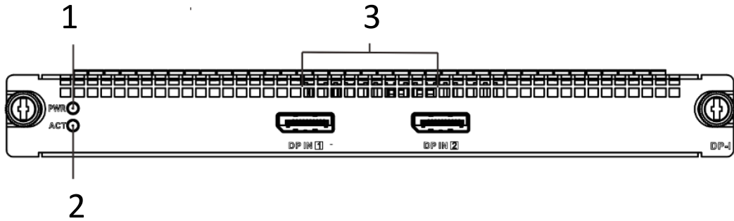
Figure 1-7 Front View of DP Input Board
