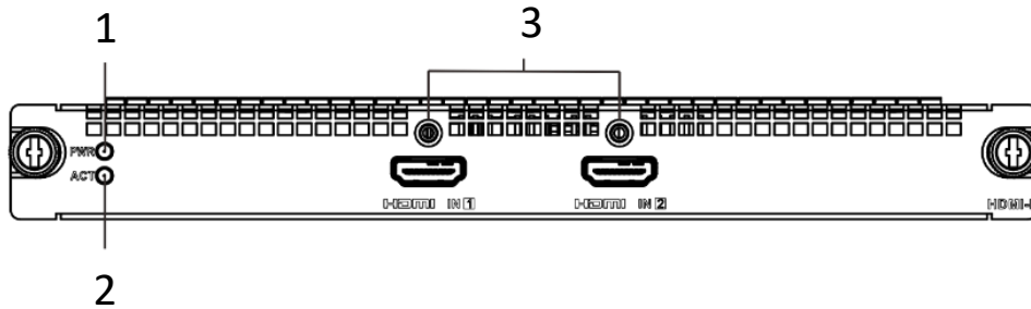
Figure 1-6 Front View of HDMI UHD Input Board
