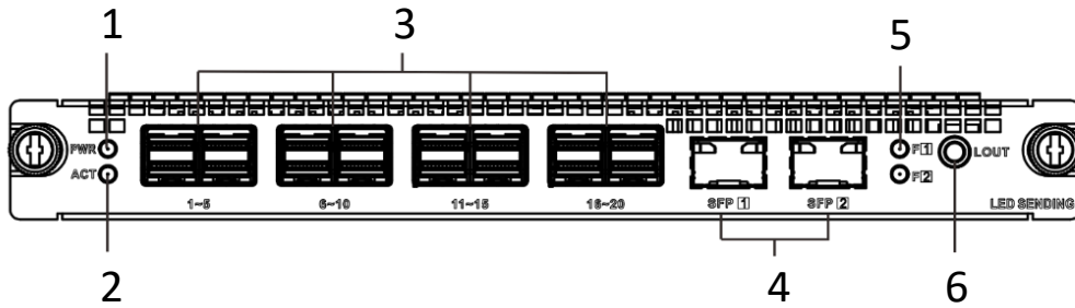
Figure 1-14 Front View of LED Sending Card
