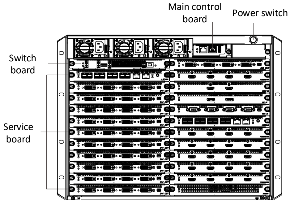
Figure 1-2 Rear View of Device
