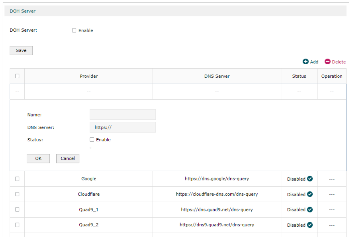
Figure 6-2 Configure DOH
