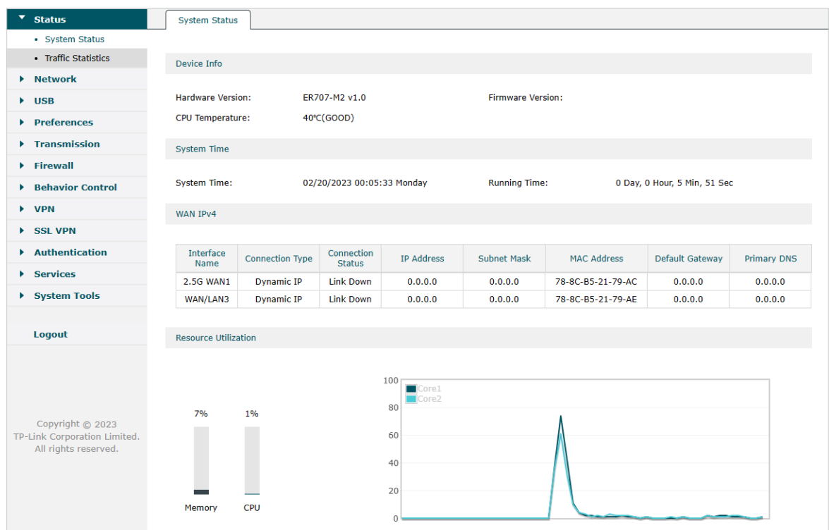
Figure 2-4 Web Interface
