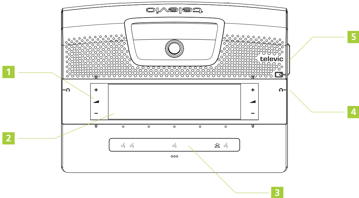
Figure 1-7 Top view of the Confidea FLEX
