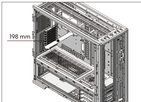
CPU Height Clearance
