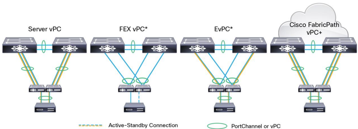
Figure 7. Cisco Nexus 2000 Series Fabric Extenders Design Scenarios, from Left to Right: Server vPC, Fabric Extender vPC, EvPC, and vPC+
