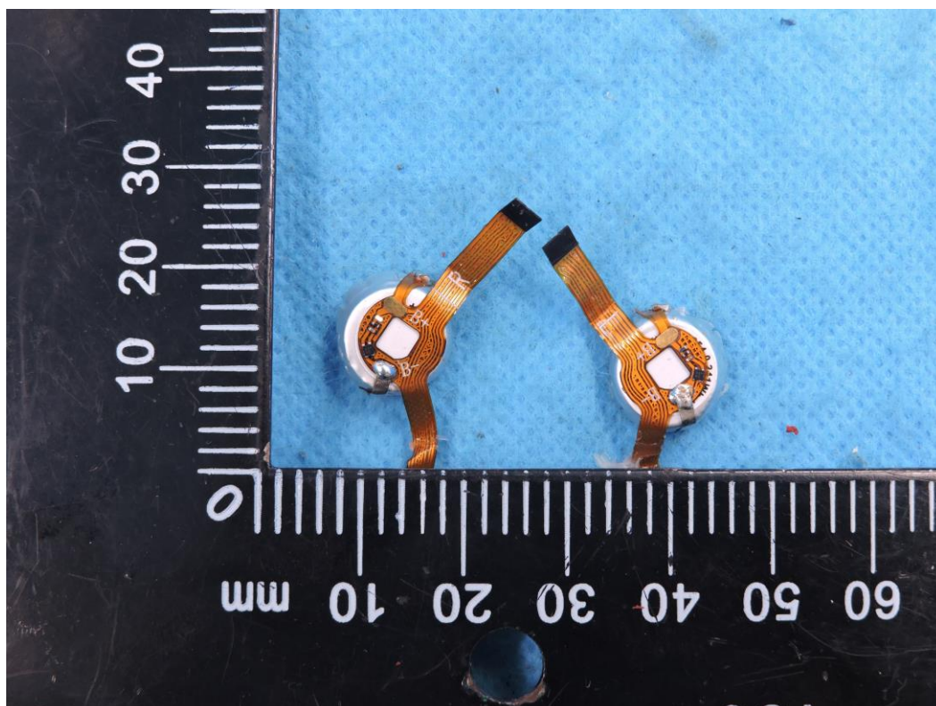
Photo 22: PCB view
