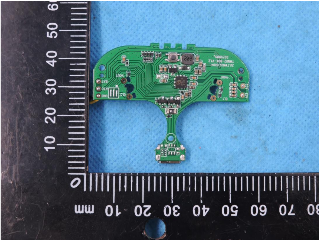
Photo 14: PCB view
