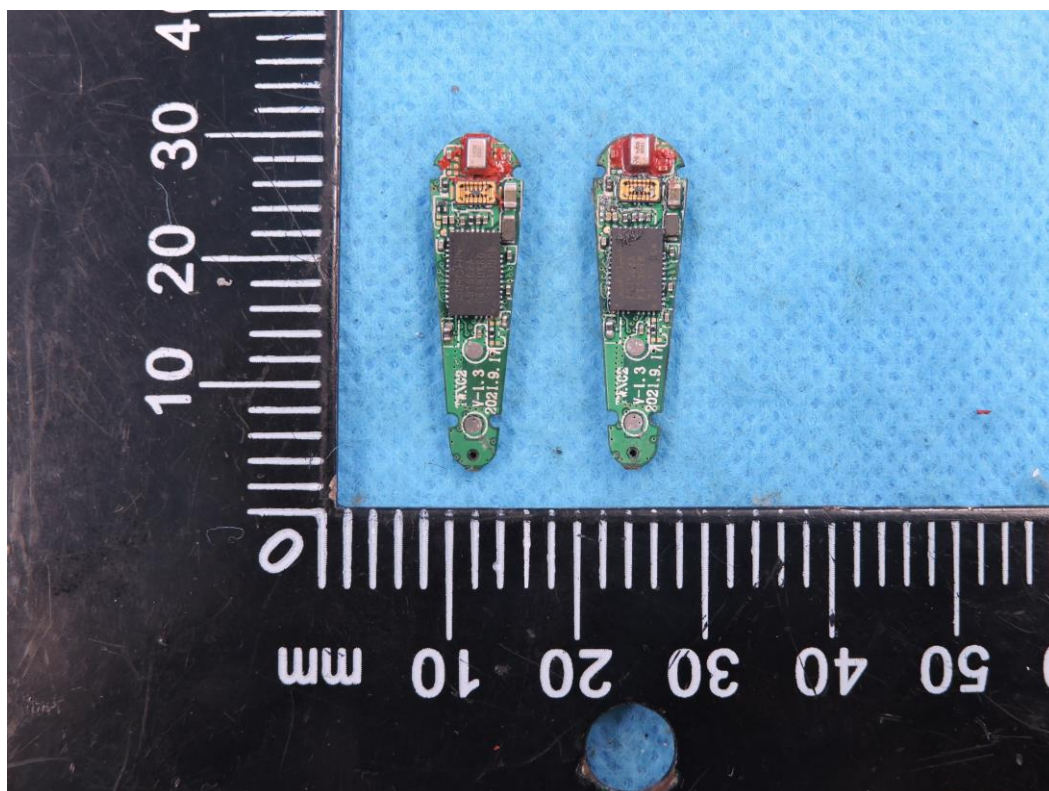
Photo 18: PCB view
