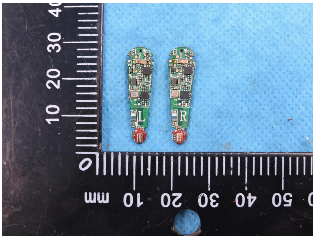
Photo 20: PCB view
