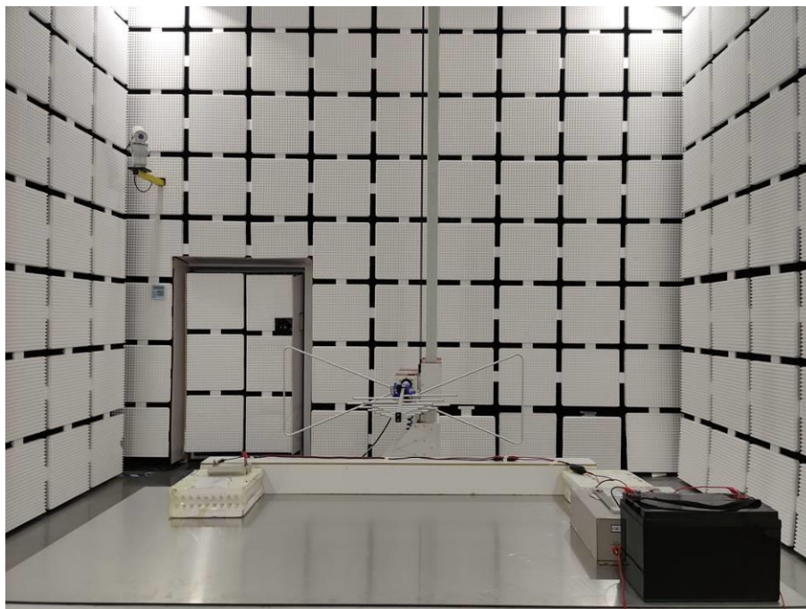
Broadband and narrowband radiated disturbances test view
