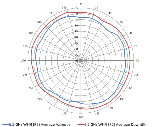
6.5 GHz Wi-Fi antenna patterns (horizontal)
