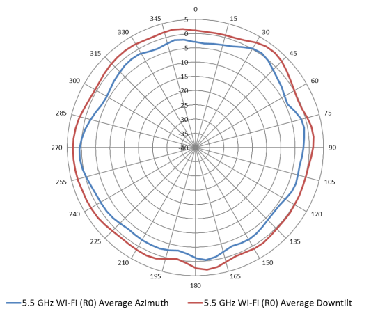
5.5 GHz Wi-Fi antenna patterns (horizontal)
