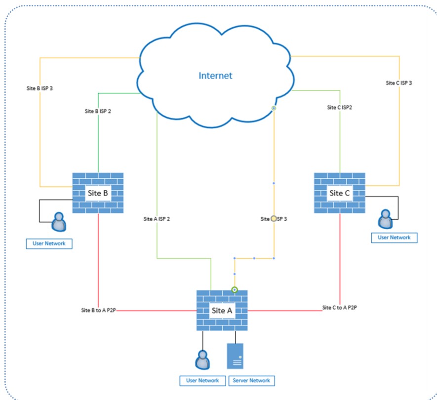
Fig. 1 – ICSA Labs SD-WAN Network Diagram
