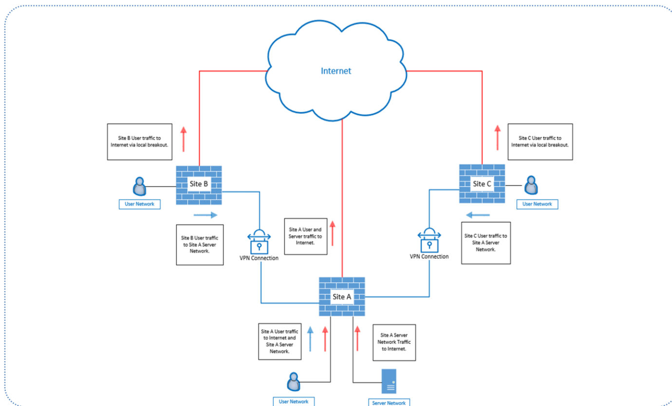
Fig. 2 – ICSA Labs SD-WAN Traffic Flows
